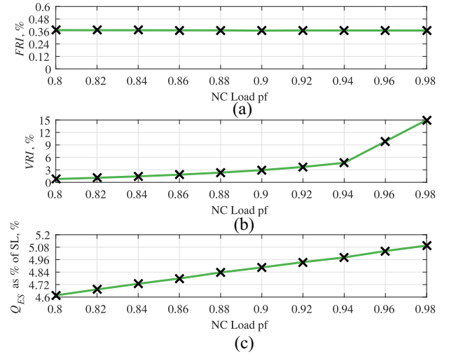
Fig. 15. Impact of load power factor on (a) FRI (7), (b) VRI (6) for mains and NC load, and (c) total reactive capacity of the compensators/ESs expressed as a percentage of the SL rating.
